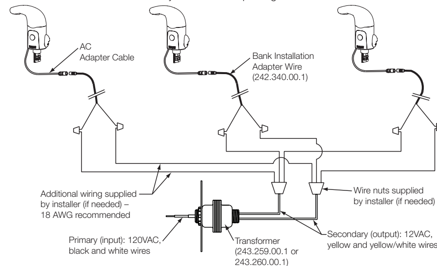
Figure 2. Example Wiring Diagram
